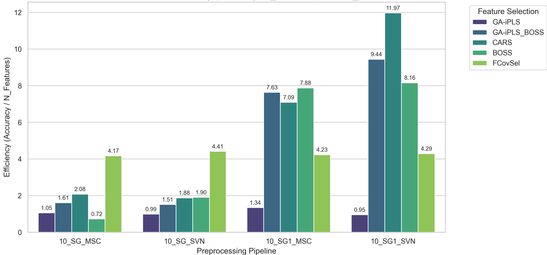
Feature Selection Efficiency (Accuracy/ N_Features) - Indian_pines
